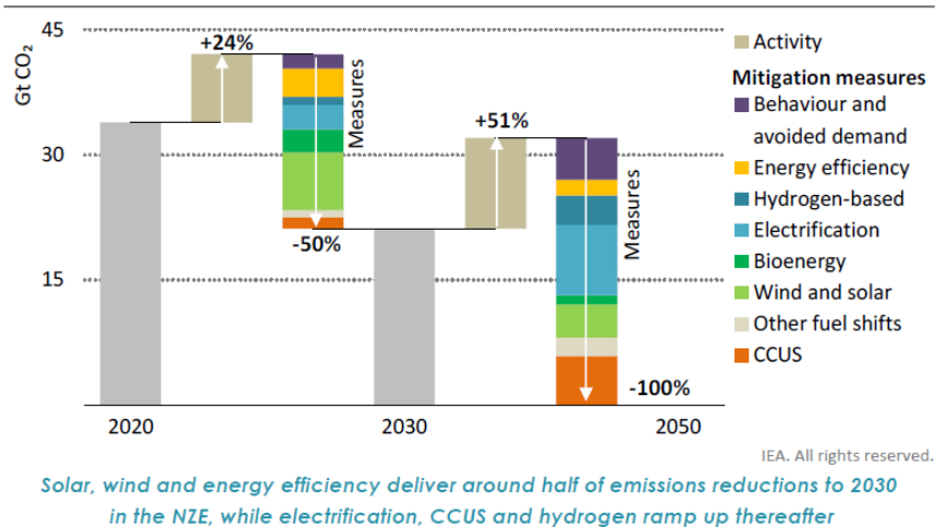
Figure 2.12 ▶ Emissions reductions by mitigation measure in the NZE, 2020-2050
