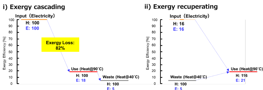
図 II -25 Exergy cascading V.S. Exergy recuperating
